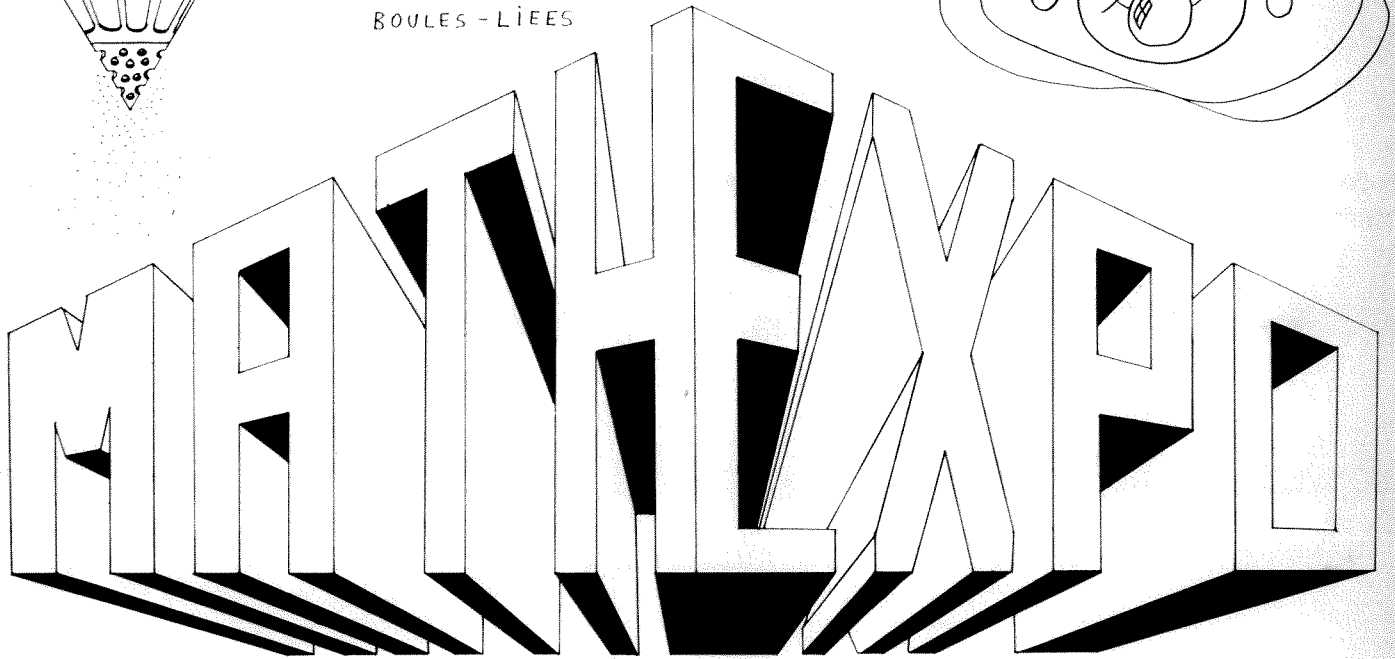
PROBABILITES
